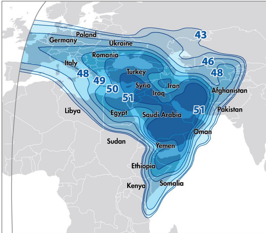
ABS-2 | MENA | 43–51 dBW 51 Ku-Band Transponders Polarization: Linear (H&V)
