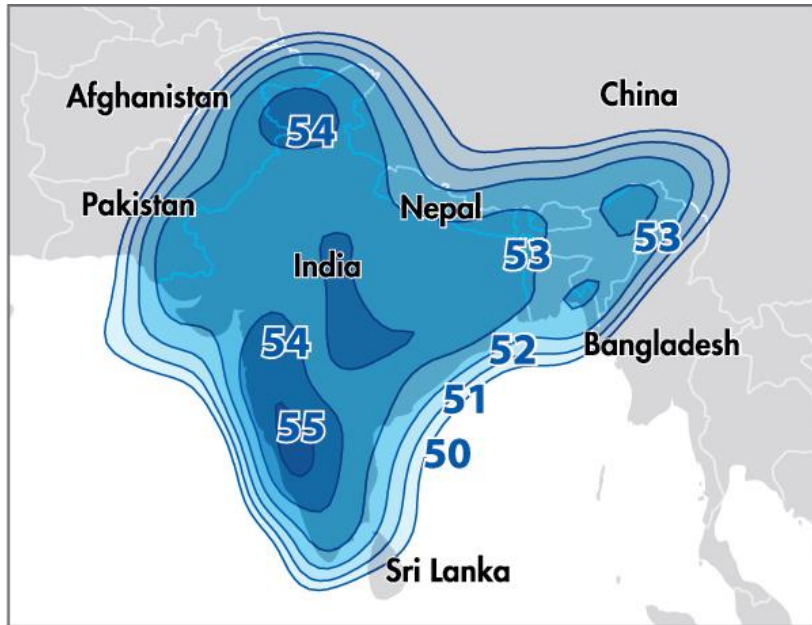
ABS-2 | South Asia | 50–54 dBW 51 Ku-Band Transponders Polarization: Linear (H&V)
