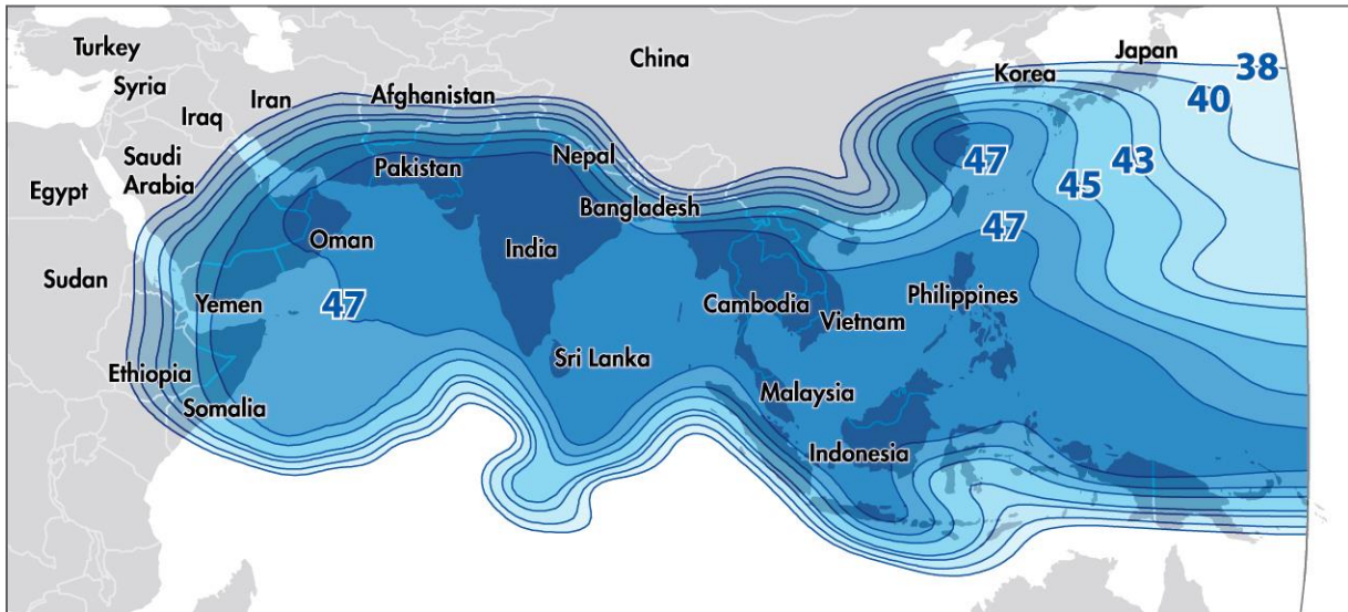
ABS-2 | Southern | 38–47 dBW 51 Ku-Band Transponders Polarization: Linear (H&V)
